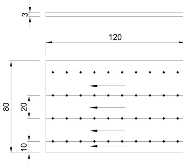
Görsel 8.12: Markalama
