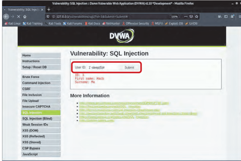
Görşel 8.12: Time Based SQL Injection atak sorgusu
